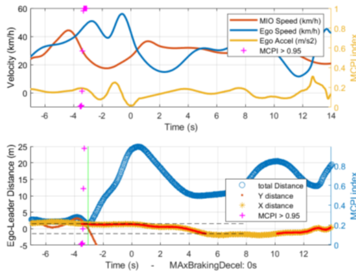
Figure 32: Example of a safety-critical event. Maximum braking deceleration corresponds to T=0s
