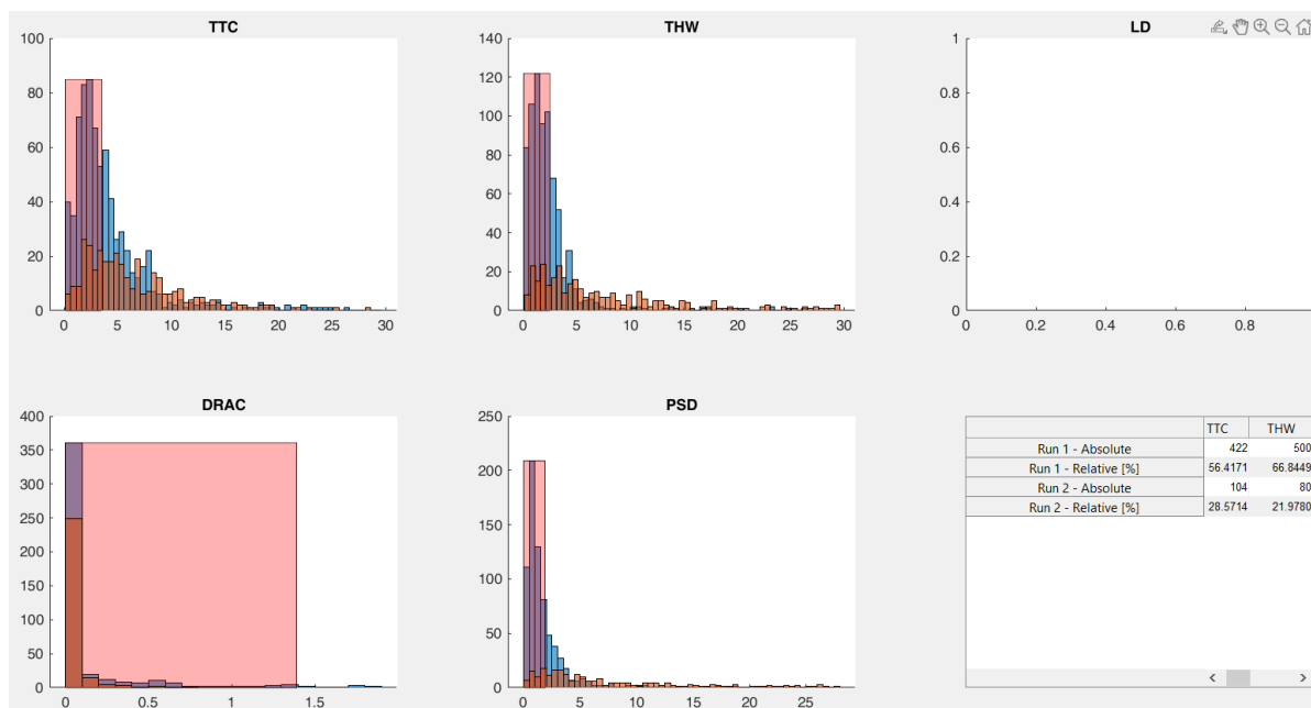
Figure 31: Evaluation Overview Cyclist
