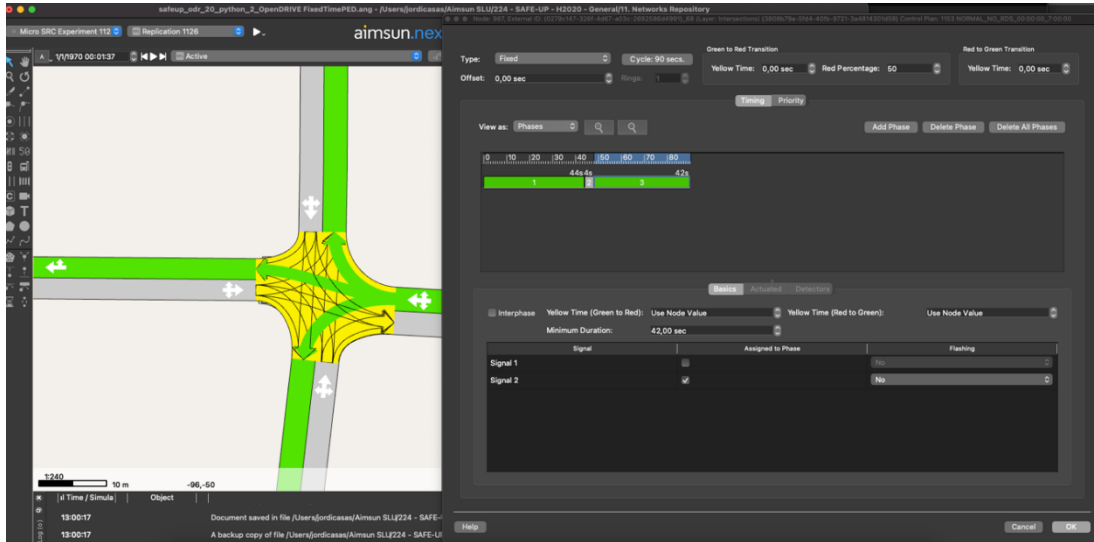
Figure 10: Example of Traffic signal control plan
